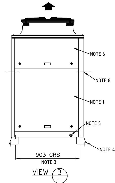
CLEARANCE DETAILS
